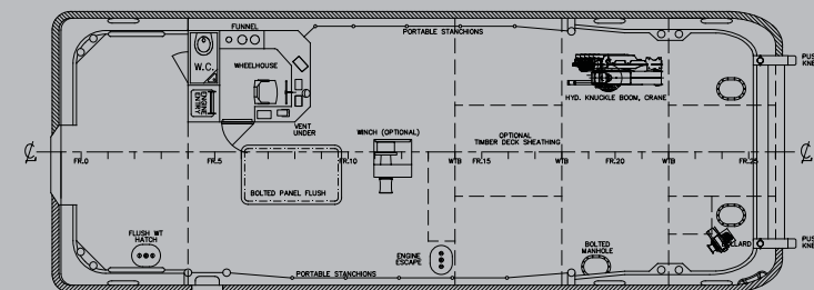
PLAN ON MAIN DECK
