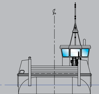
BODY PLAN
