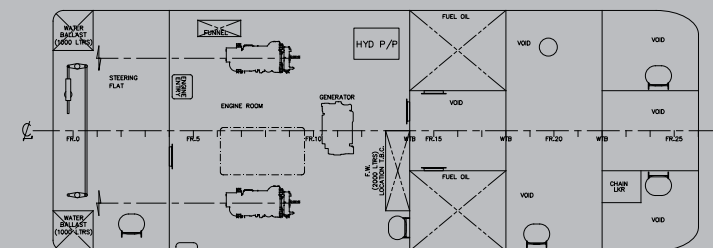
PLAN BELOW MAIN DECK
