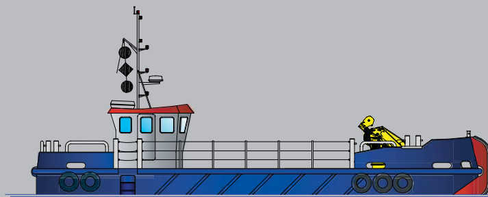
PROFILE TO WATERLINE
